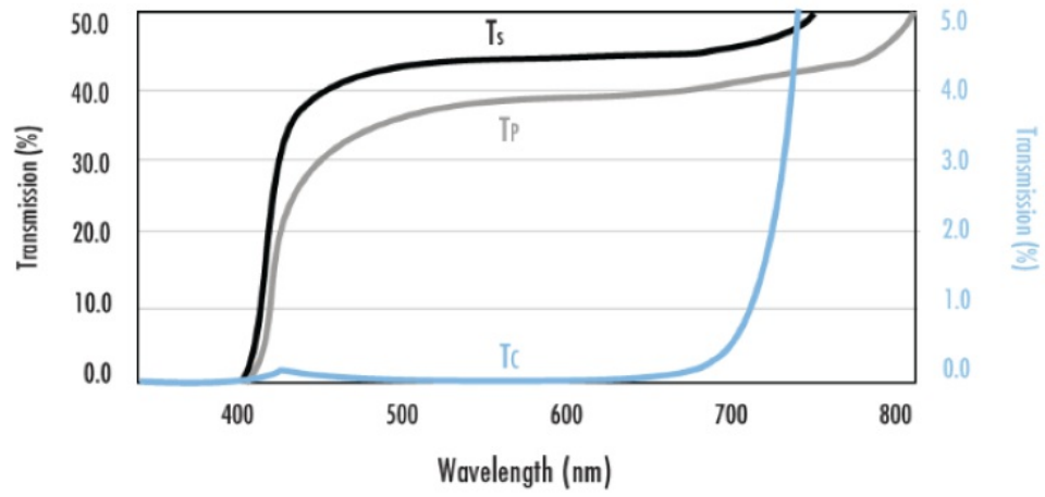
XP44 – Linear Polarizer
