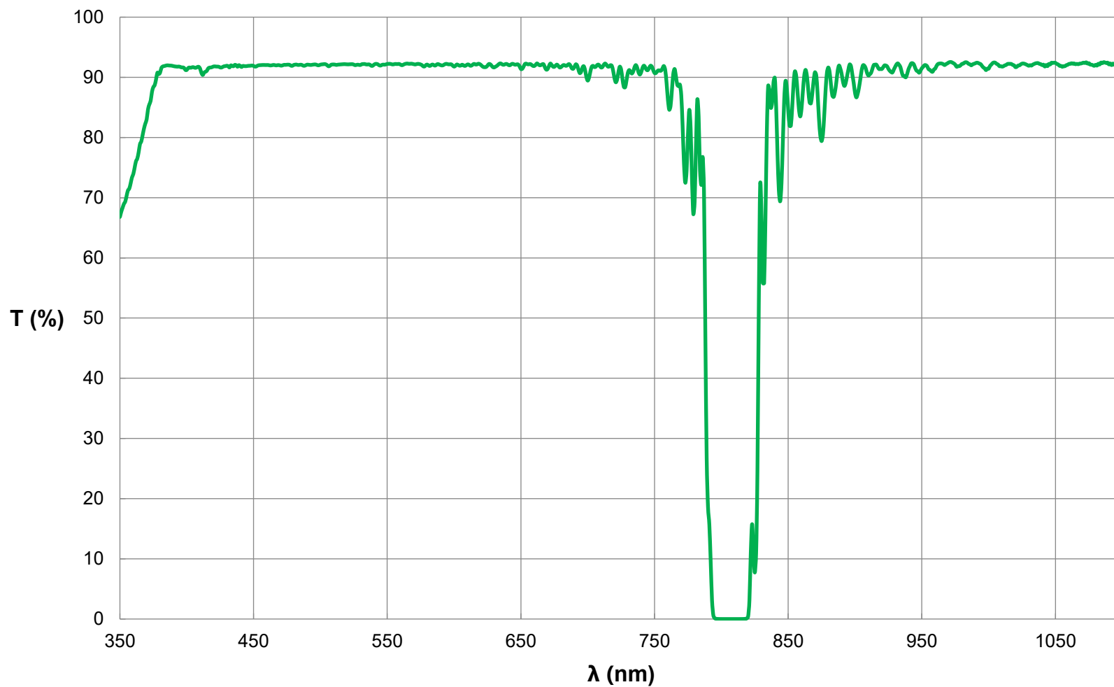
Everix Ultra-Thin OD 4 Notch Filter, 808nm, 12.5mm Diameter FOR REFERENCE ONLY
